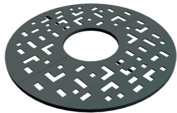
Pangaia TS-03 • diameter - 1800 mm • inner diameter - 600 mm • height - 50 mm
