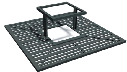
Uno TS-06 • length - 1800 mm • width - 1800 mm • height - 50 mm • hole for trunk - 600×600 mm • height for trunk - 490 mm
