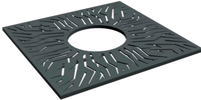
Uno TS-02 • length - 1500 mm • width - 1500 mm • height - 50 mm • inner diameter - 500 mm
