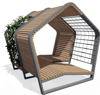
Fresh GB-03 • length - 2260 mm • width - 2000 mm • height - 2080 mm
