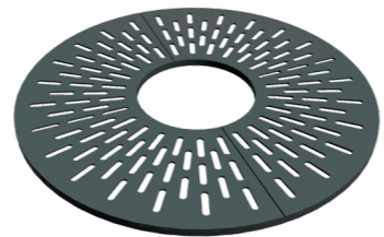
Pangaia TS-04 • diameter - 1800 mm • inner diameter - 600 mm • height - 50 mm
