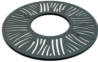
Pangaia TS-01 • diameter - 1700 mm • inner diameter - 600 mm • height - 50 mm
