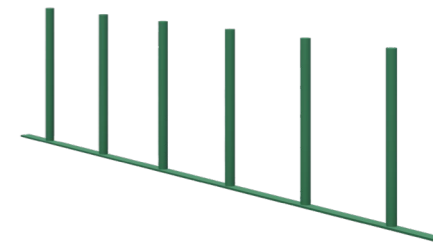
Animal DP-07 • length - 3600 mm • width - 40 mm • height - 950 mm
