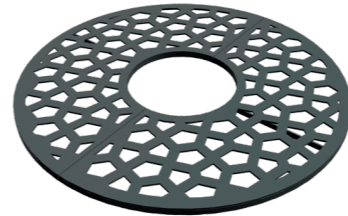
Pangaia TS-05 • diameter - 1800 mm • inner diameter - 600 mm • height - 50 mm
