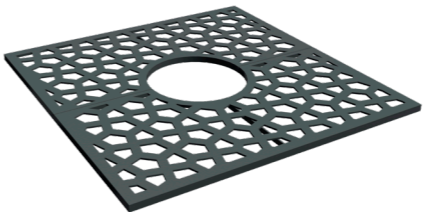
Uno TS-05 • length - 1800 mm • width - 1800 mm • height - 50 mm • inner diameter - 600 mm
